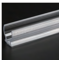
PC Profile 1000(+5)x10.5x13.7mm(LxWxH) Accessories: Screw M3x15mm
